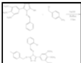
Fig. 3. The synthesis procedure of the title compound.
