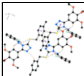
Fig. 2. A packing view of the title compound. The intermolecular C—H...N, C—H...S and C—H... \pi interactions are shown as dashed lines.
