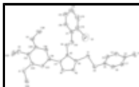
Fig. 1. The structure of the title compound, showing the atomic numbering scheme. Non-hydrogen atoms are shown with 30% probability displacement ellipsoids. Hydrogen atoms have been omitted for clarity.
